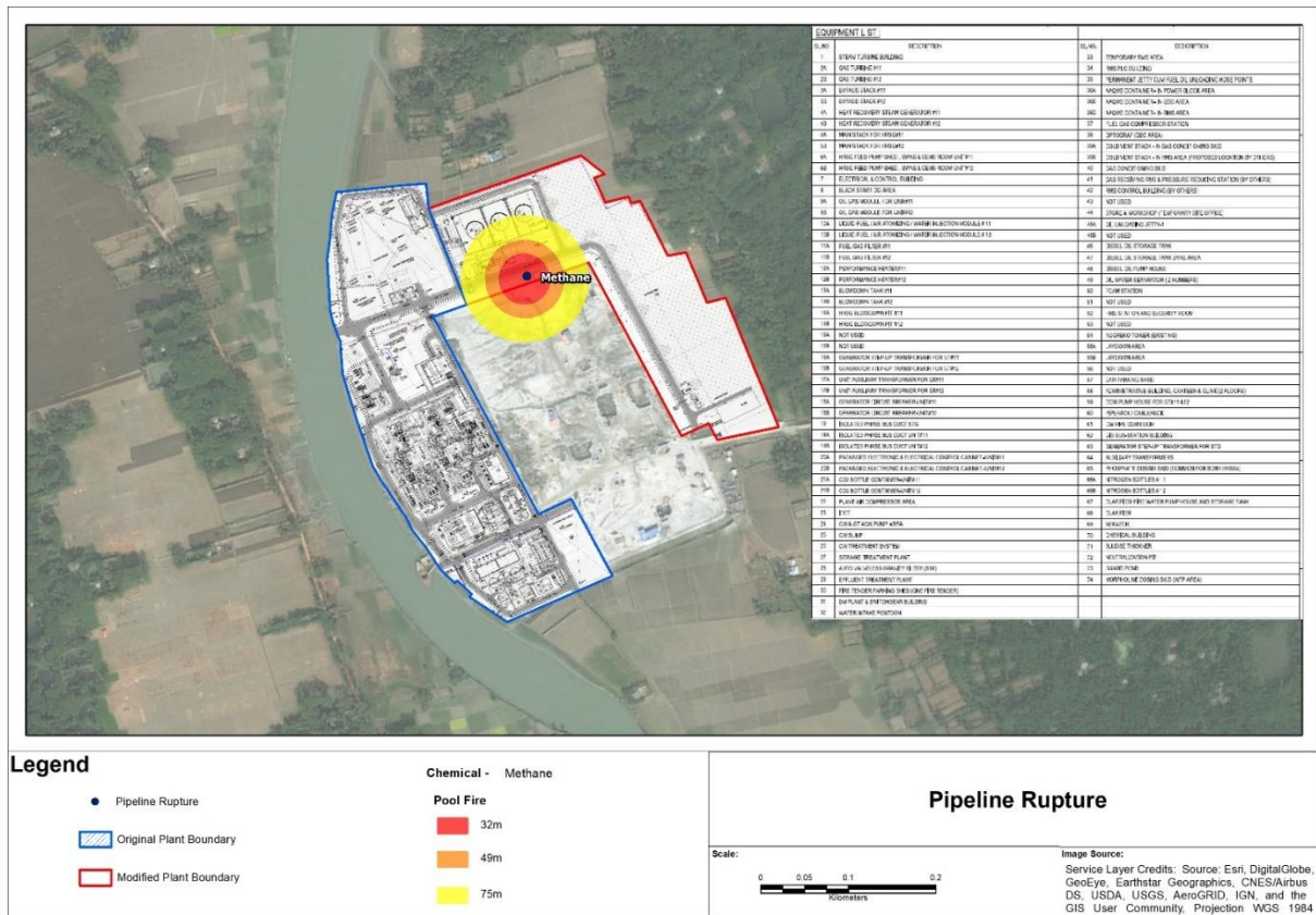
Figure 5.10 Threat Zone Plot – Temporary Gas Pipeline Rupture
