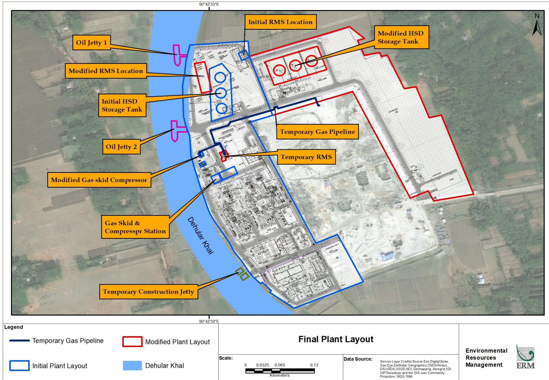
Figure 1.3 Final PlantLayout Plan –showing the Modification
