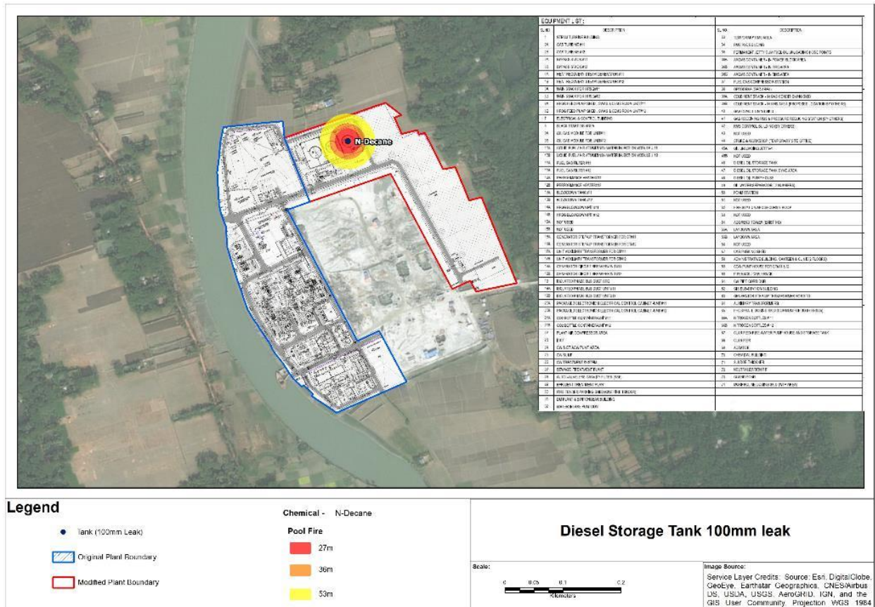
Figure 5.5 Threat Zone Plot –100mm leak
