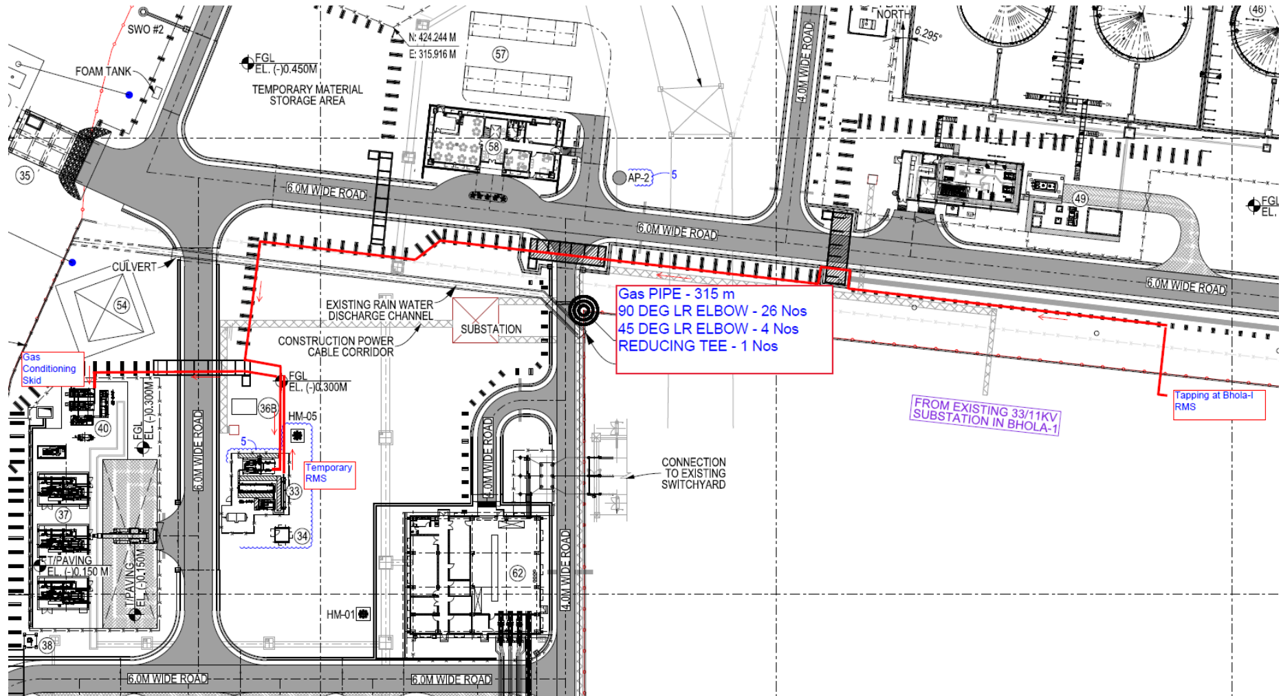
Figure 1.5 Temporary Gasline and RMS
