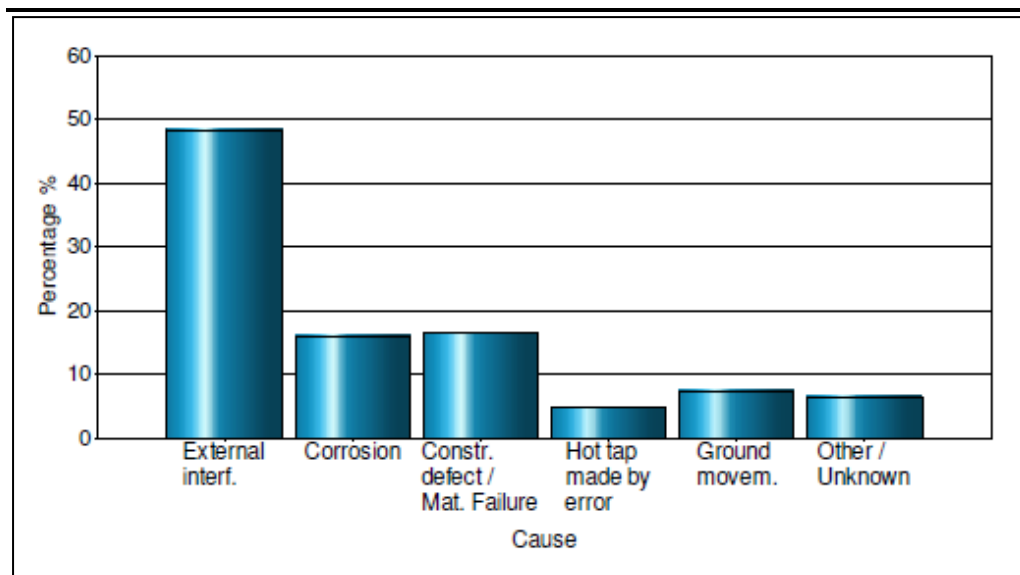
Figure 5.3 Gas Pipeline Failure – Distribution of Incident & Causes
