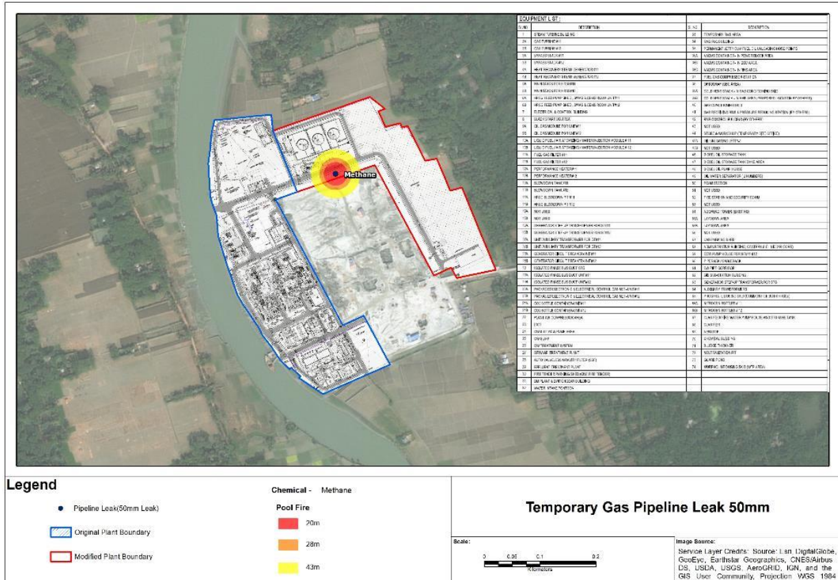
Figure 5.9 Threat Zone Plot – Temporary Gas Pipeline Leak (50mm dia)
