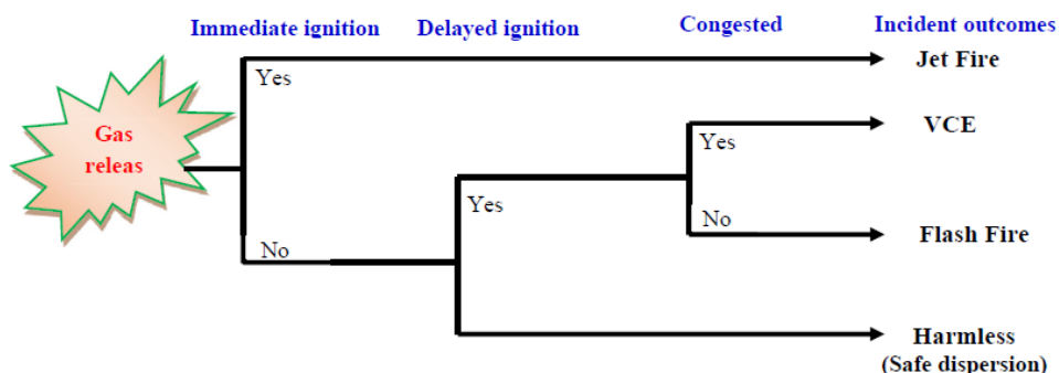
Figure 5.7 Natural Gas Release – Potential Consequences
