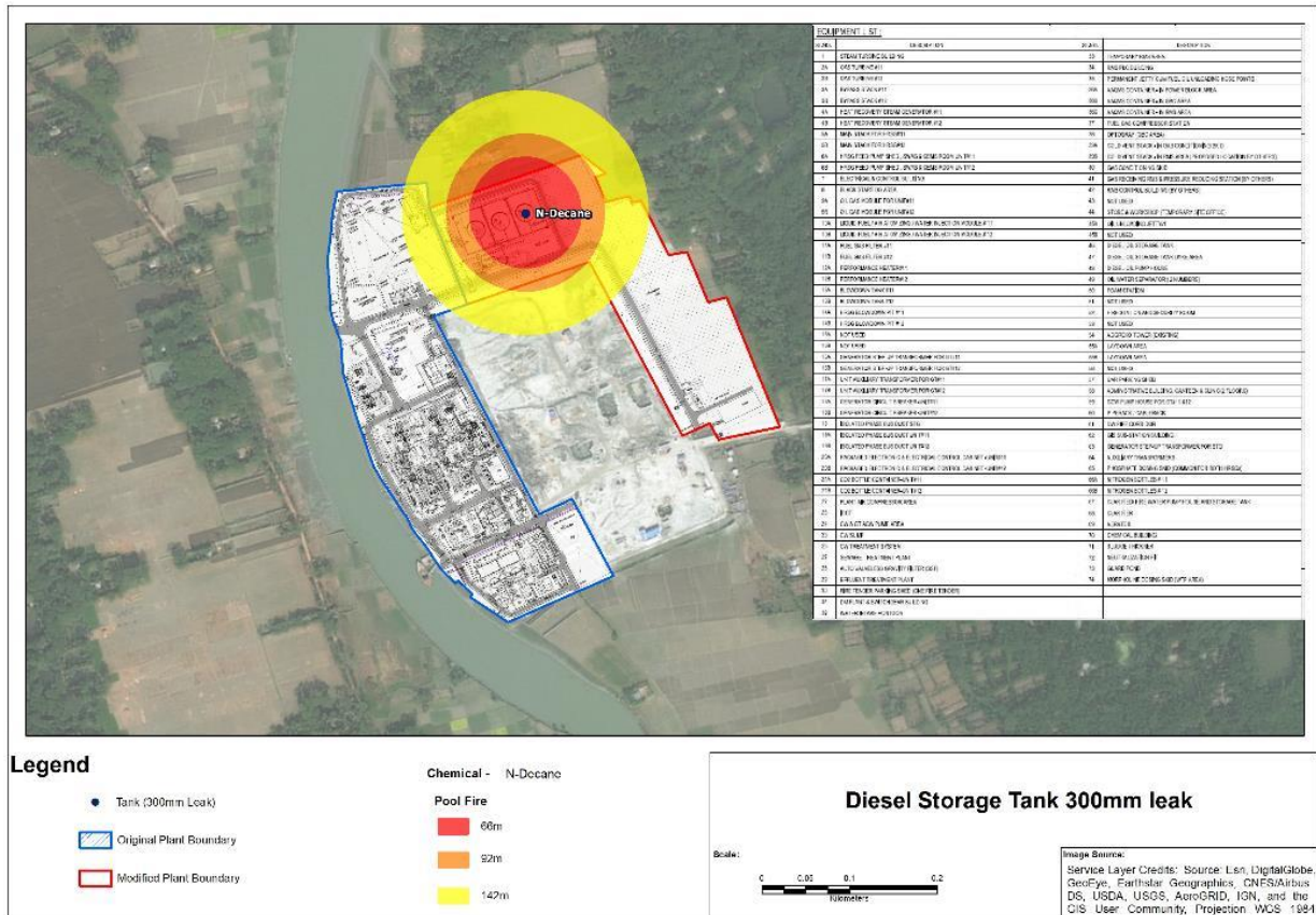
Figure 5.6 Threat Zone Plot –300 mm leak (Worst Case)
