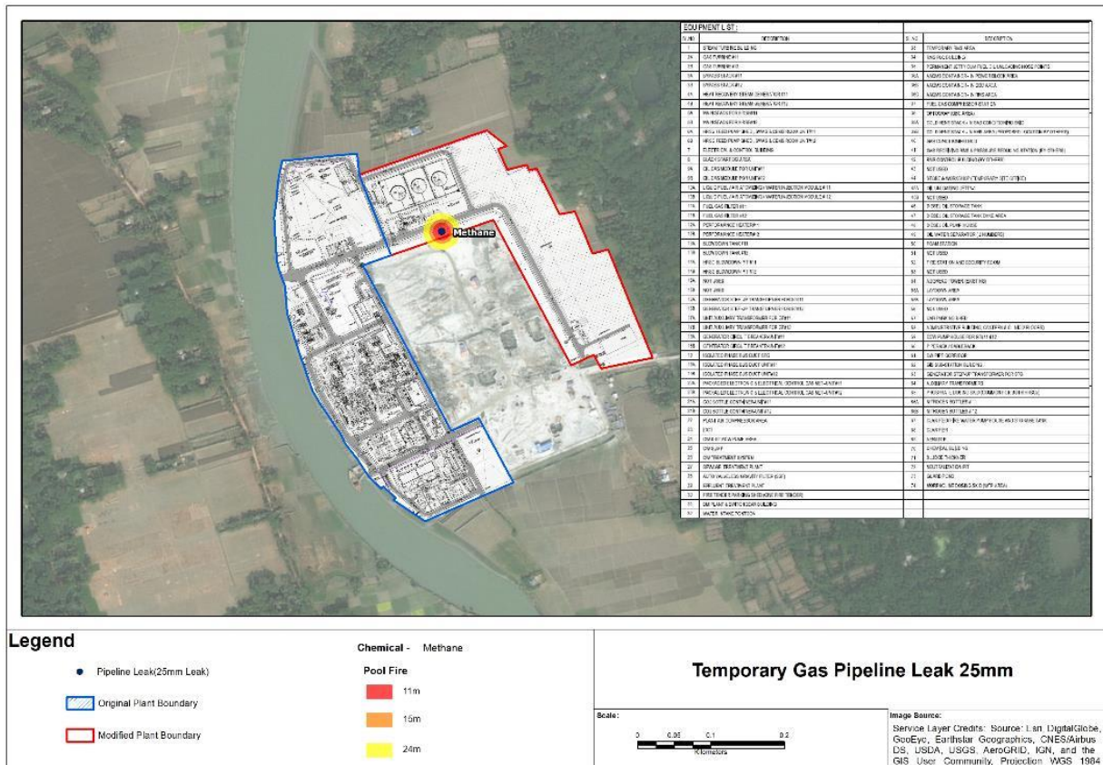
Figure 5.8 Threat Zone Plot – Temporary Gas Pipeline Leak (25mm dia)
