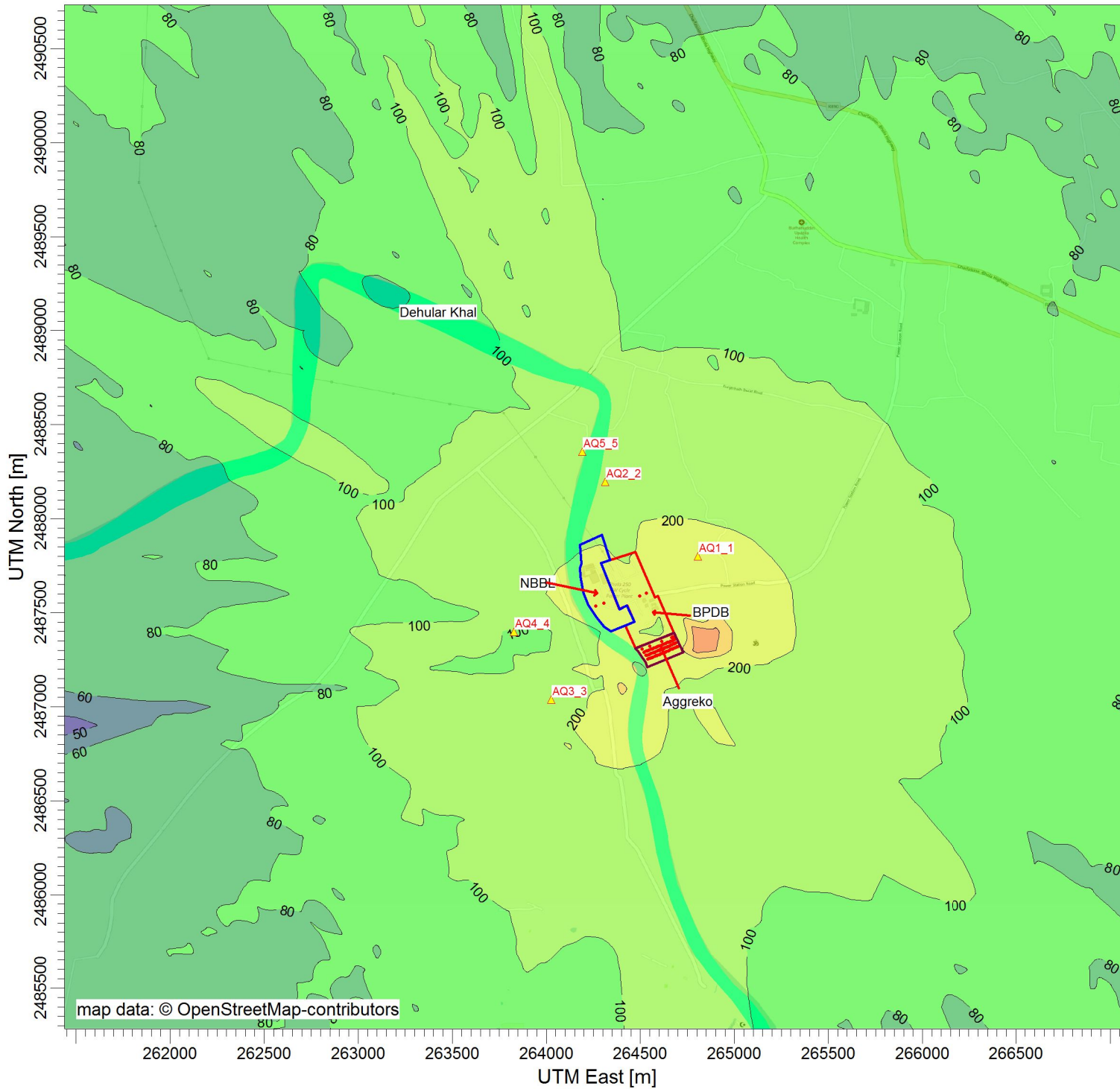
PLOT FILE OF HIGH 1ST HIGH 1-HR VALUES FOR SOURCE GROUP: AGGREKO
