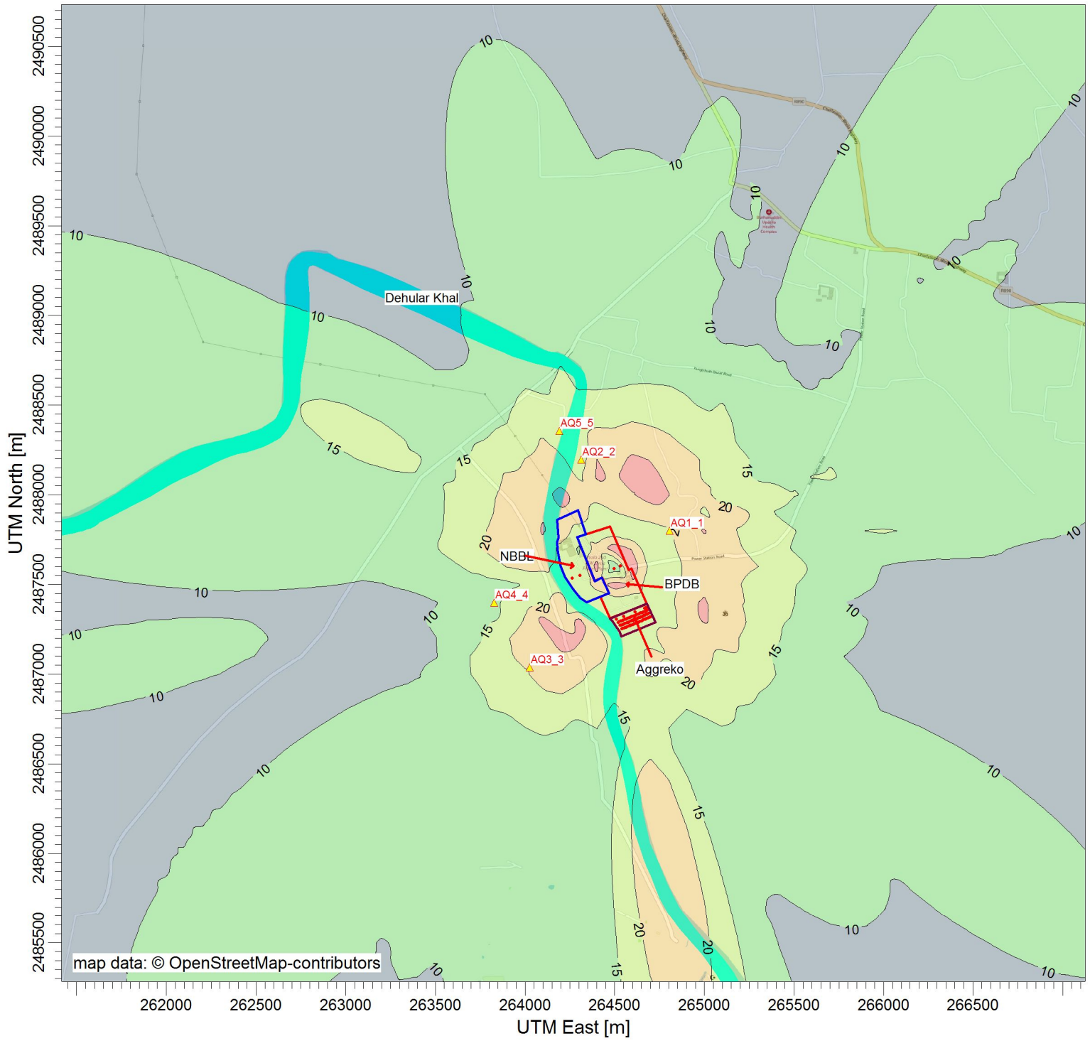
PLOT FILE OF HIGH 1ST HIGH 1-HR VALUES FOR SOURCE GROUP: BPDB Max: 28 [ug/m^3] at (264600.00, 2487600.00)
