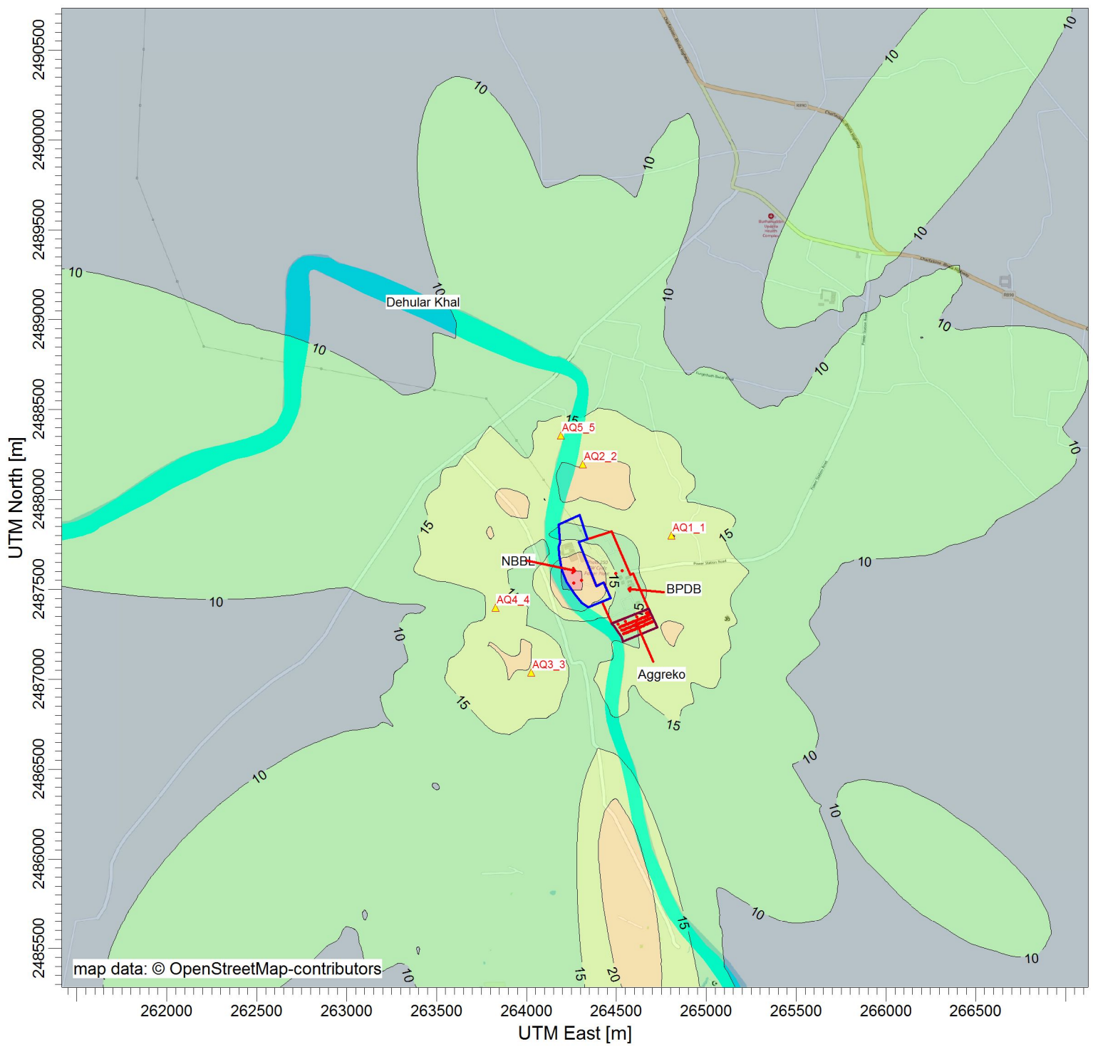
PLOT FILE OF HIGH 1ST HIGH 1-HR VALUES FOR SOURCE GROUP: NBBL Max: 26 [ \mu\text{g}/\text{m}^3 ] at (264200.00, 2487600.00)
