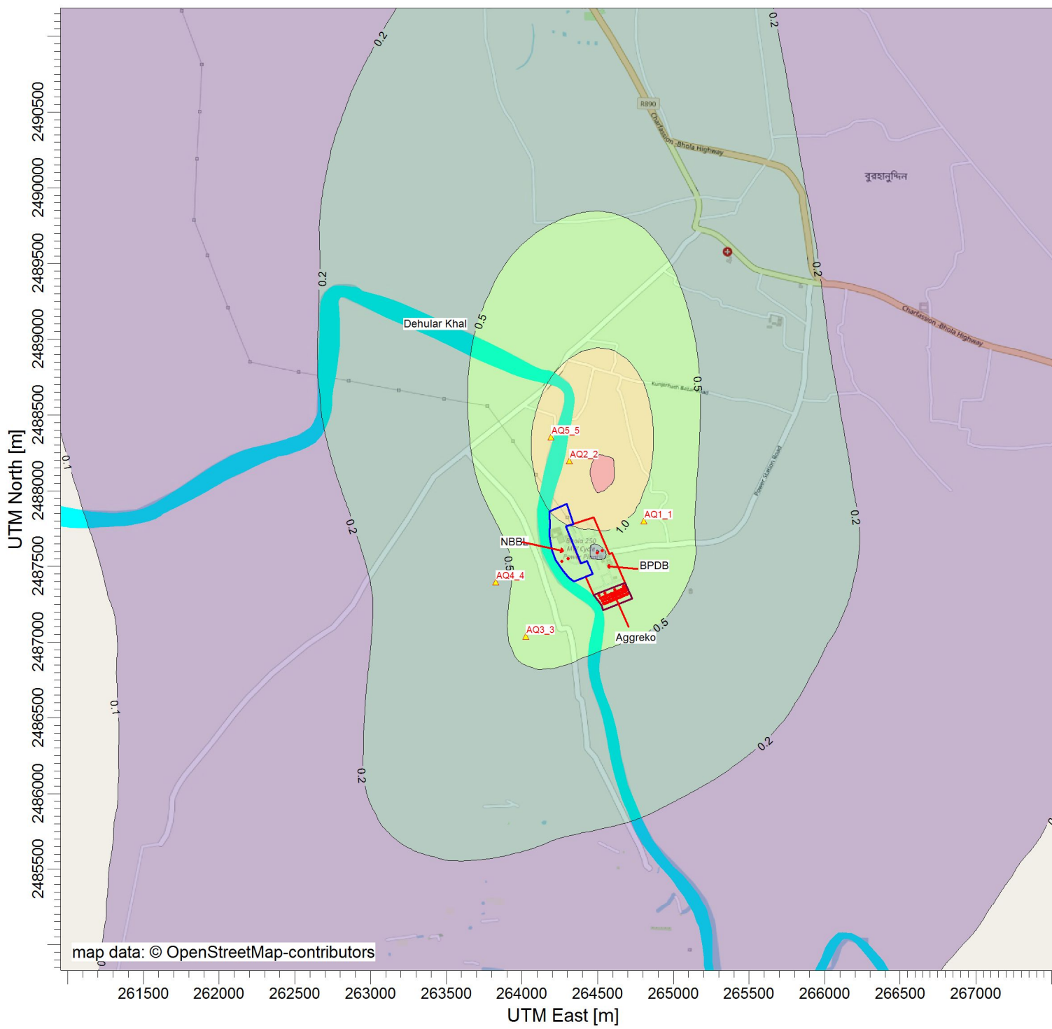
PLOT FILE OF ANNUAL VALUES AVERAGED ACROSS 1 YEARS FOR SOURCE GROUP: BPDB Max: 2.2 [ug/m^3] at (264500.00, 2488100.00)
