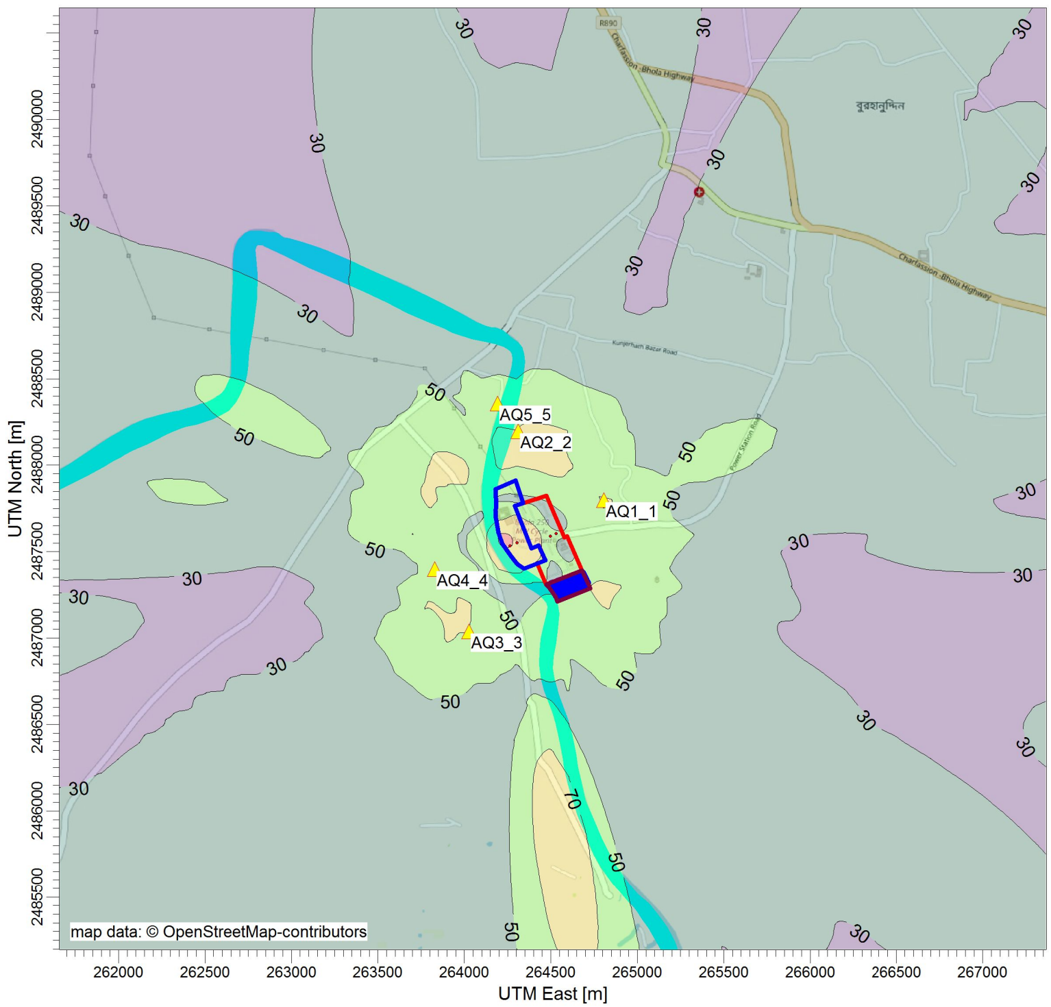
PLOT FILE OF HIGH 1ST HIGH 1-HR VALUES FOR SOURCE GROUP: NBBL Max: 92 [ug/m^3] at (264200.00, 2487600.00)
