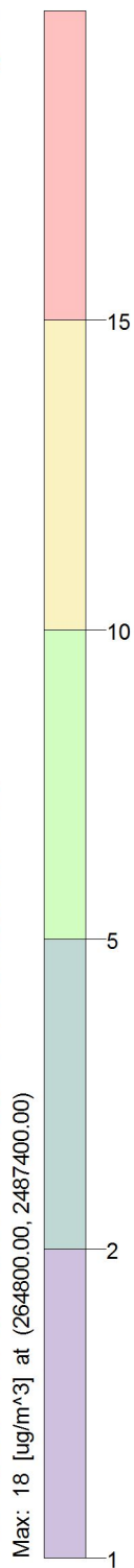
PLOT FILE OF HIGH 1ST HIGH 24-HR VALUES FOR SOURCE GROUP: ALL
